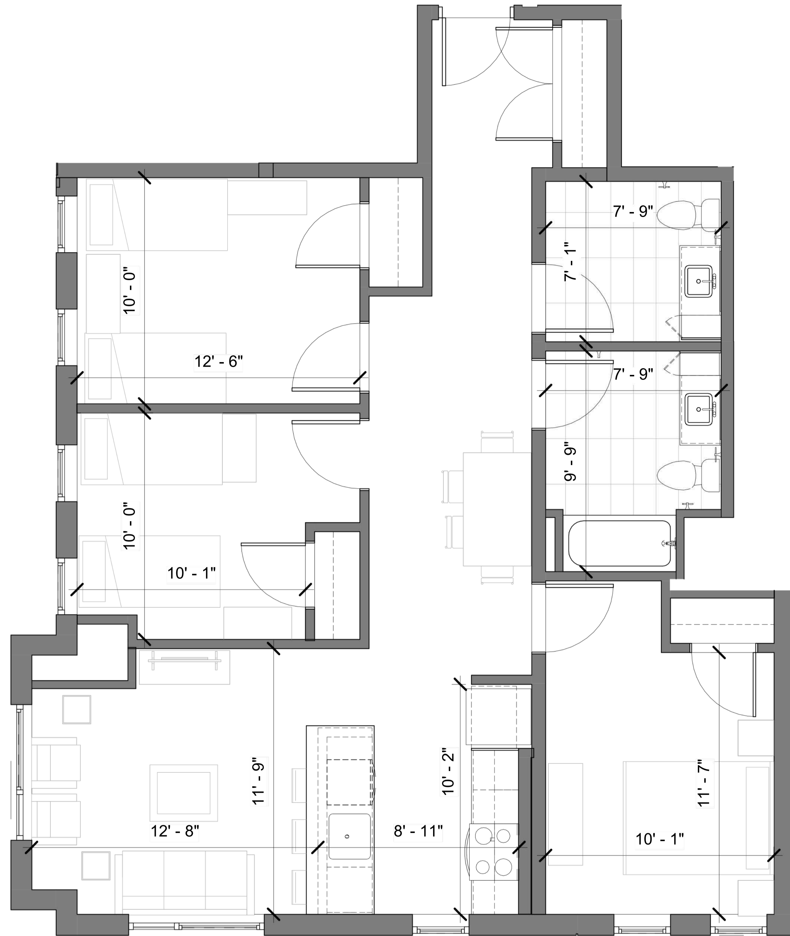
3BR TYPE A Plan -1018 SF
