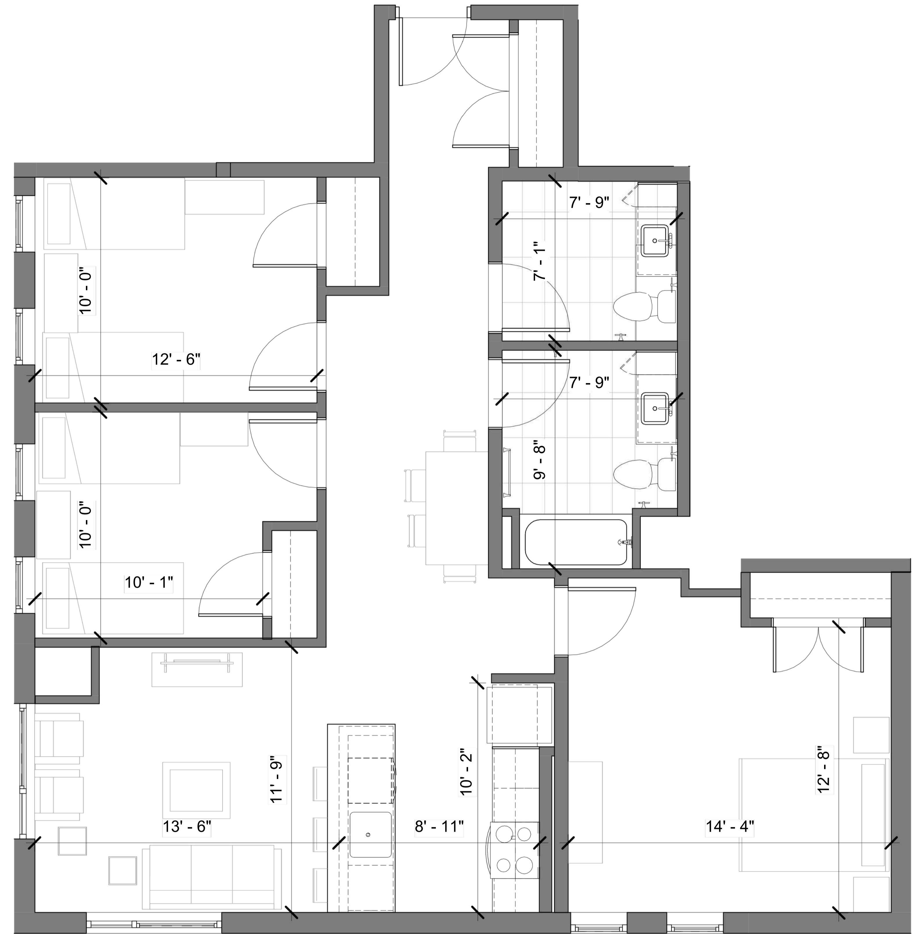
3BR TYPE A.1 Plan -1119 SF
