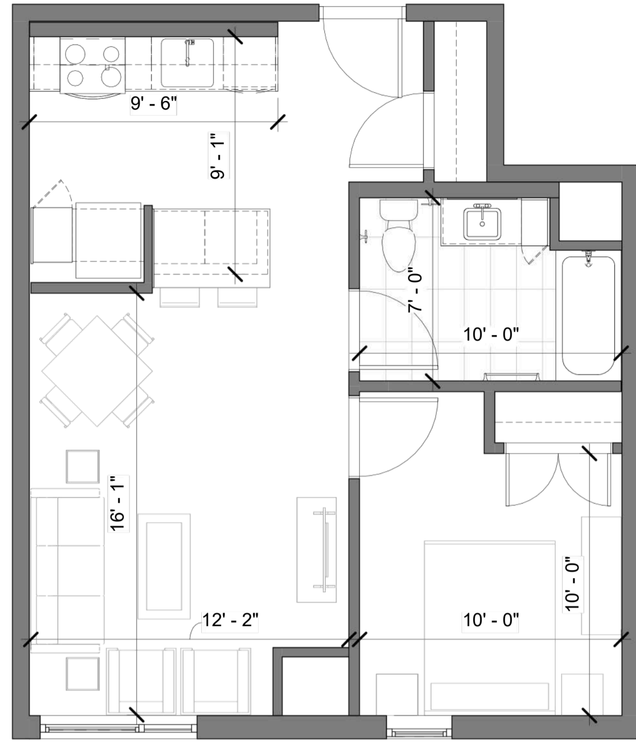
1BR TYPE A Plan -562 SF
