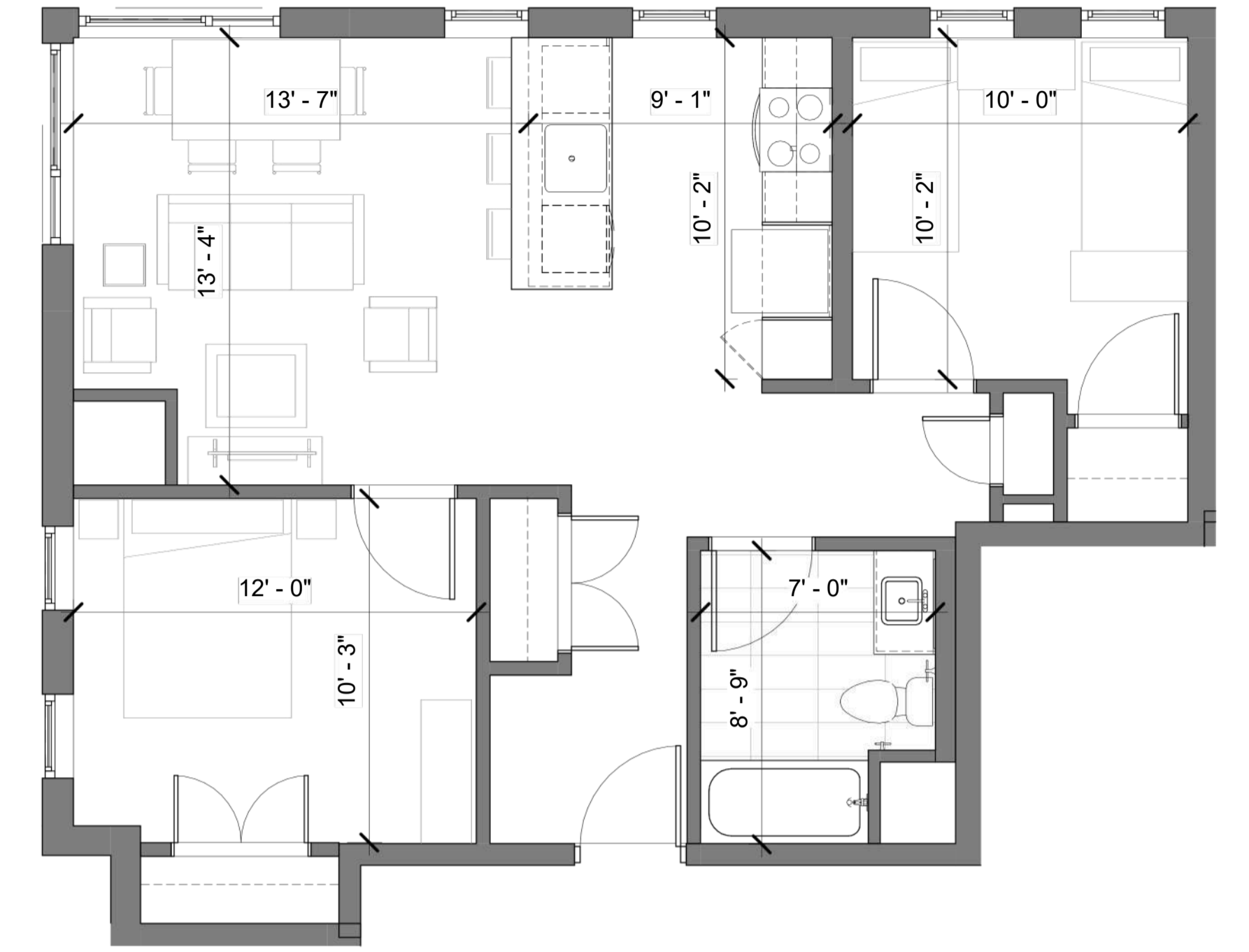
2BR TYPE B.1 Plan -720 SF
