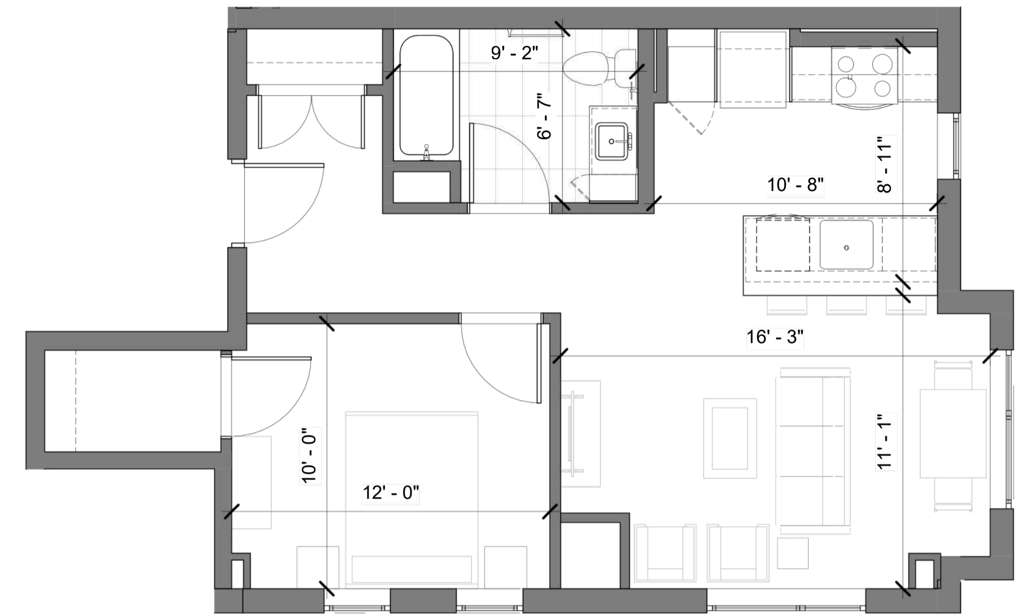
1BR TYPE C Plan - 440 SF
