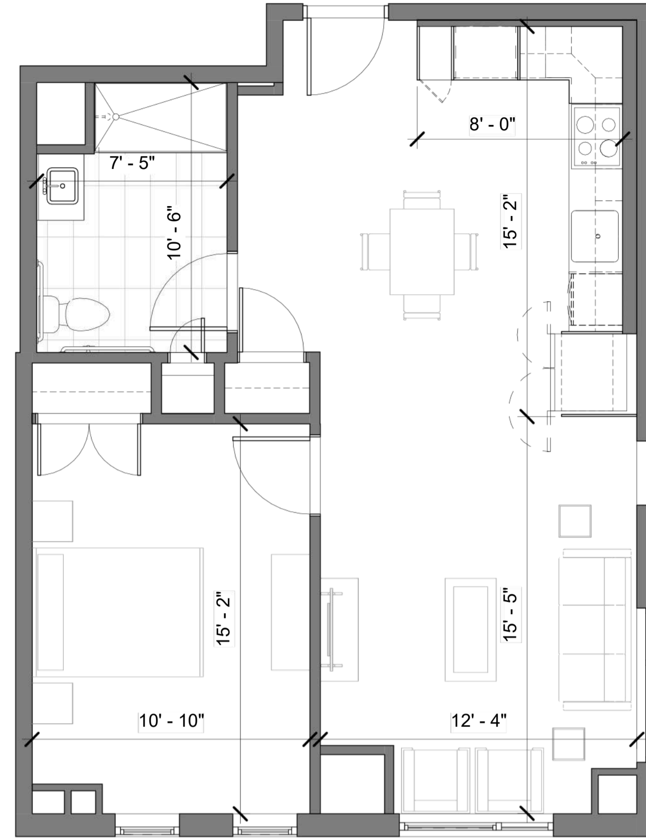
1BR TYPE B BF Plan -677 SF
